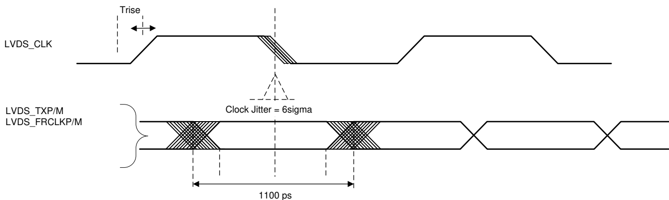
Figure 6-22. Timing Parameters
