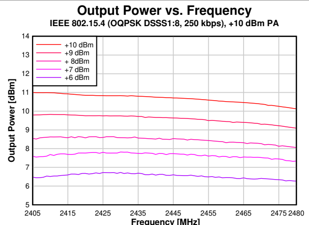
Figure 8-32. Output Power vs. Frequency (250 kbps, +10 dBm PA)
