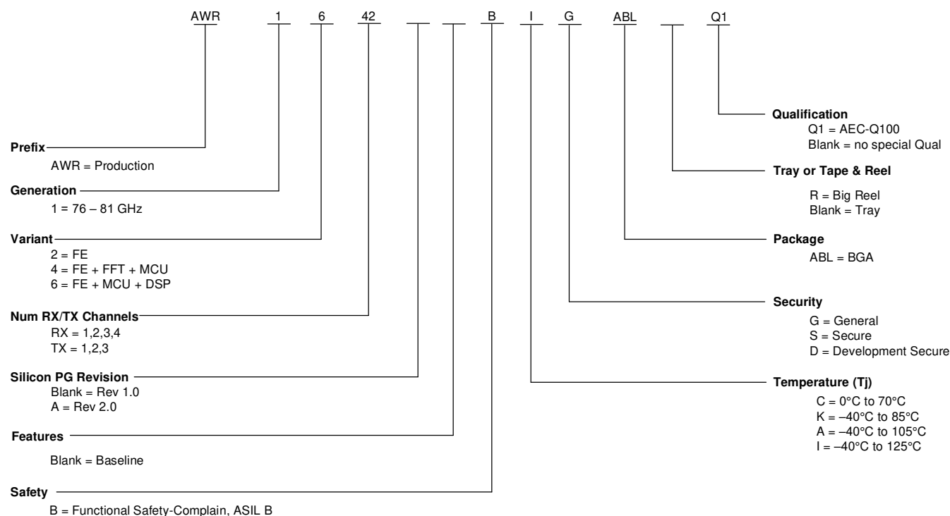
Figure 11-1. Device Nomenclature
