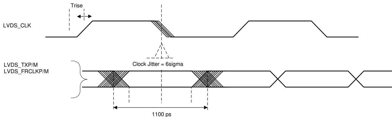
Figure 8-13. Timing Parameters
