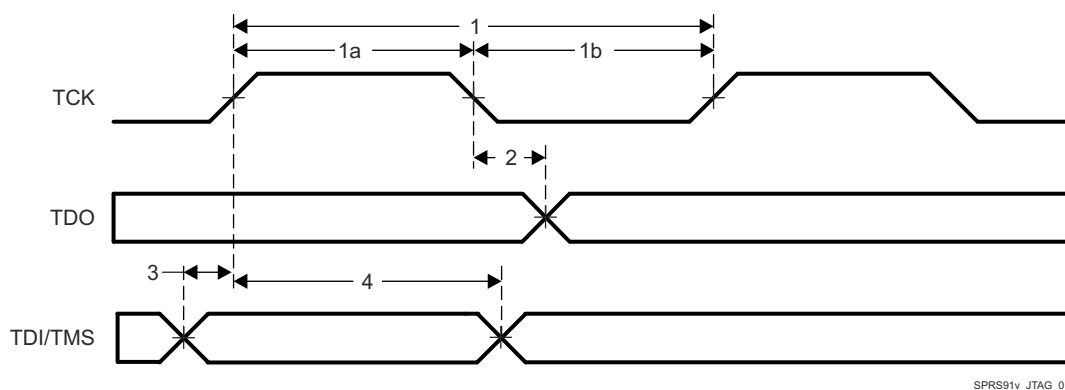
Figure 8-17. JTAG Timing
