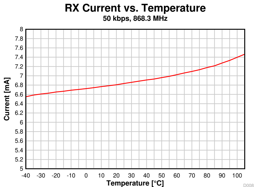
Figure 8-7. RX Current vs. Temperature (50 kbps, 868.3 MHz)
