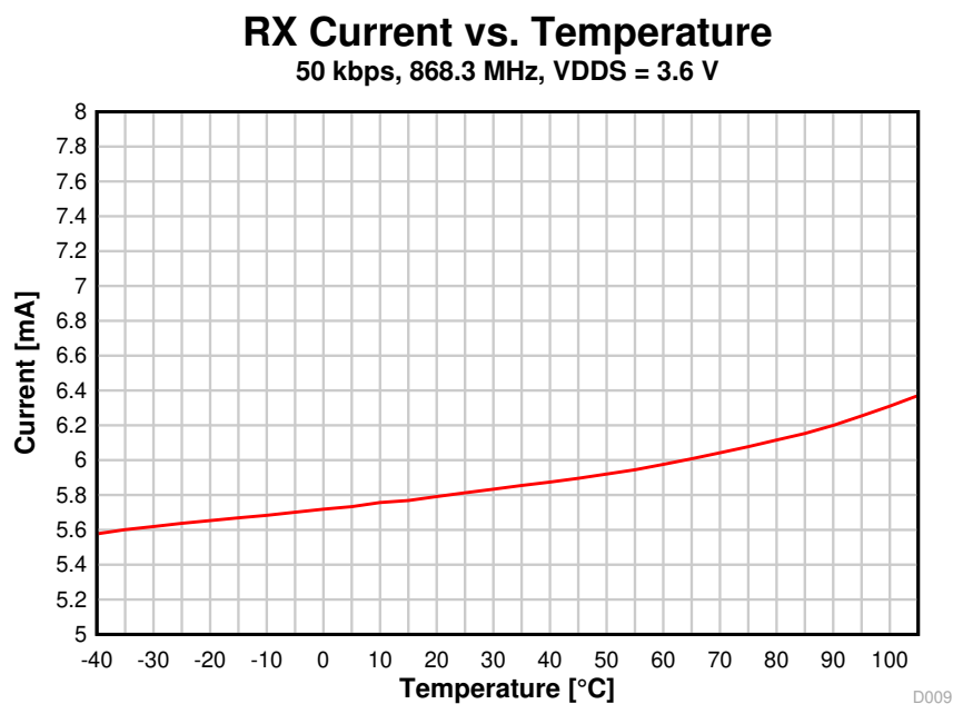
Figure 8-8. RX Current vs. Temperature (50 kbps, 868.3 MHz, VDD5 = 3.6 V)
