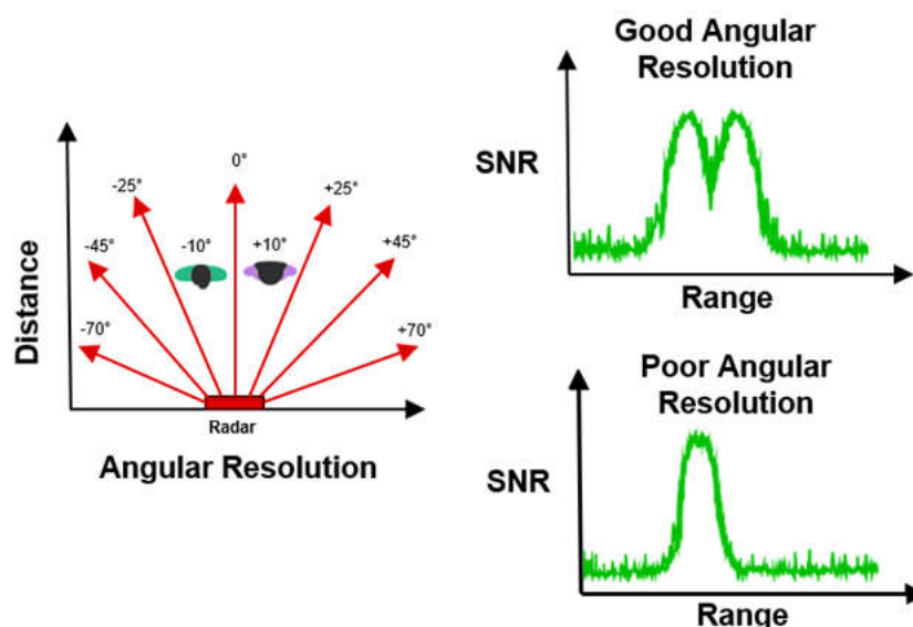
Figure 4. Top down view of Radar utilizing Angular Resolution to differentiate between two objects
