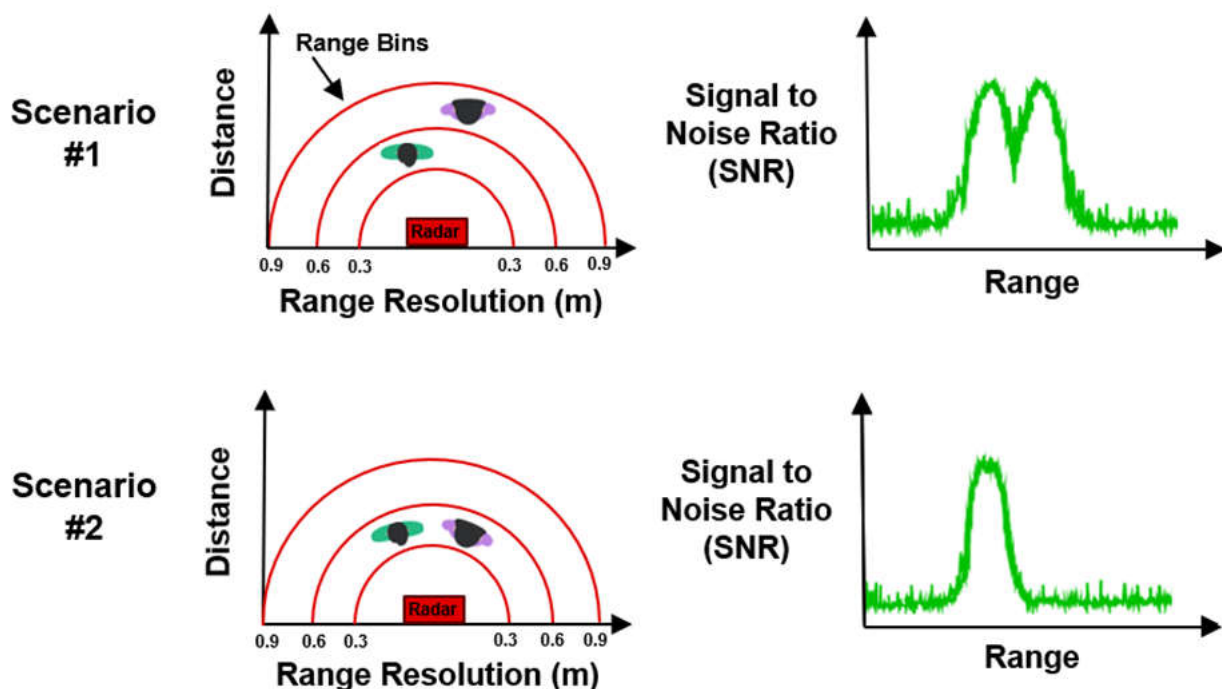
Figure 2. Top-down view of Radar differentiating between two objects using range resolution
