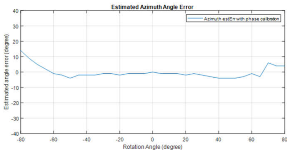
Figure 5. TI IWR6844 Angular Accuracy margin of error relative to angle
