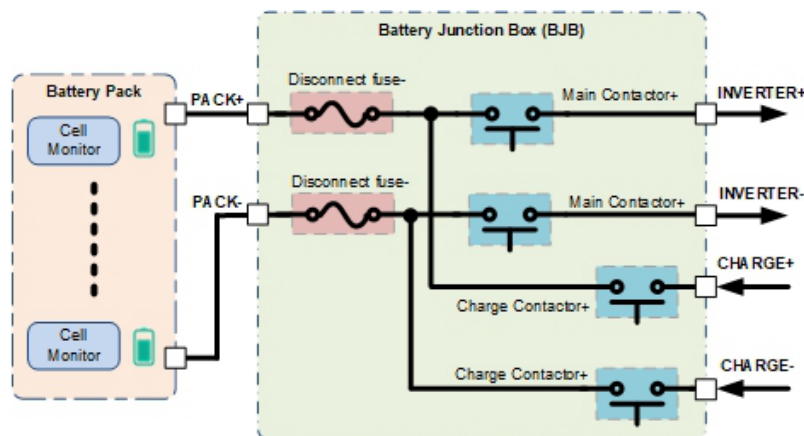
Figure 1. Battery disconnect fuse and high voltage relays in power distribution
