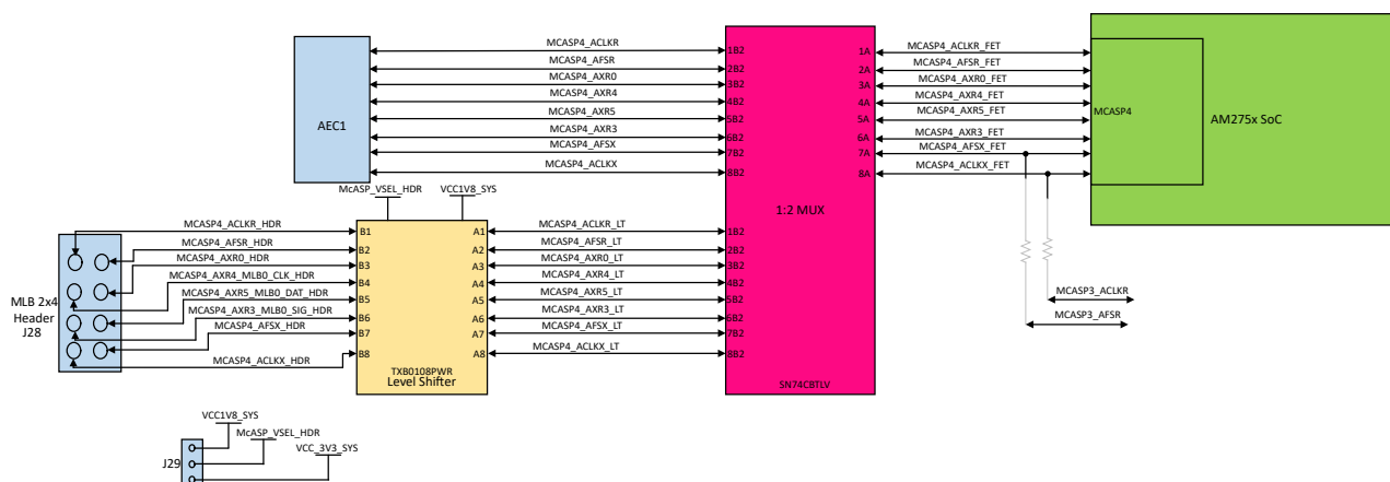
Figure 2-31. MLB Header
