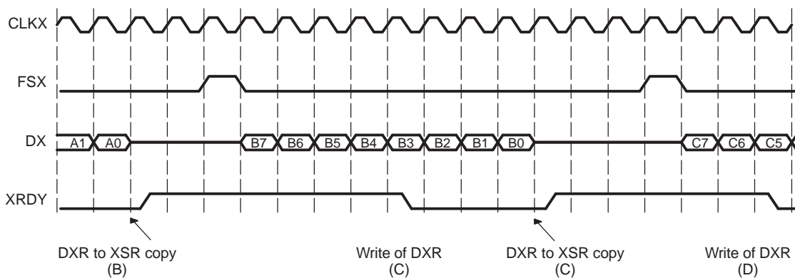
Figure 14. Transmit Operation
