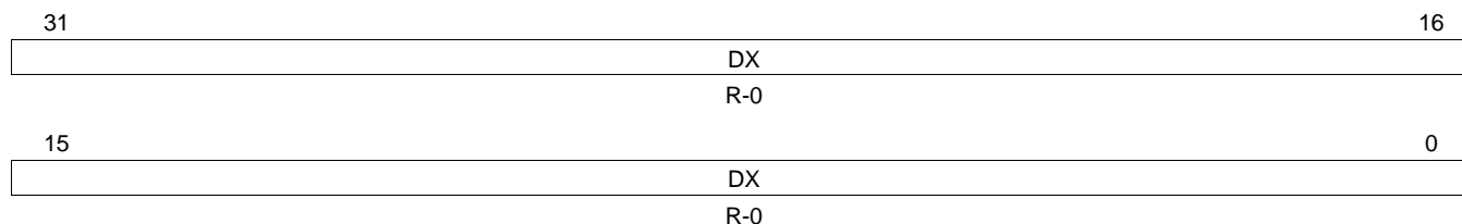
Figure 34. Data Transmit Register (DXR)
