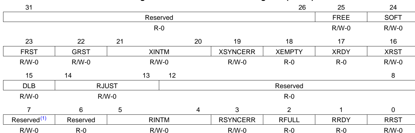
Figure 35. Serial Port Control Register (SPCR)
