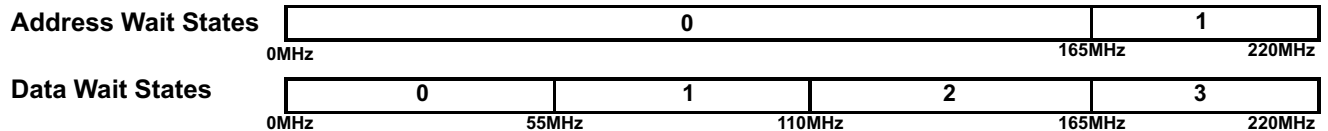
Figure 5-1. Wait States Scheme
