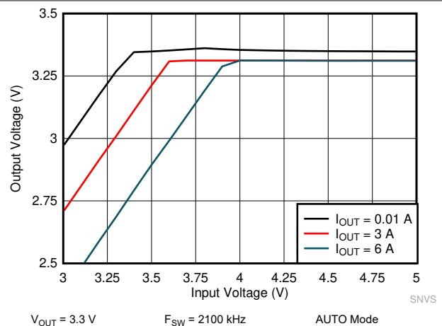
Figure 10-22. LM61460-Q1 Dropout Curve
