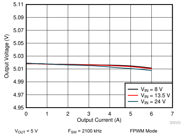
Figure 10-20. LM61460-Q1 Load and Line Regulation
