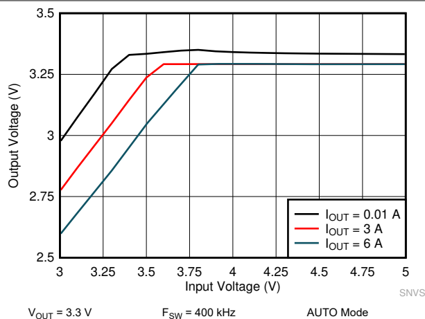
Figure 10-21. LM61460-Q1 Dropout Curve
