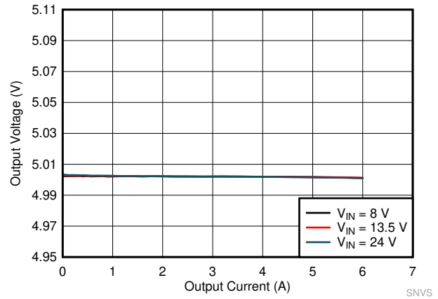
Figure 10-18. LM61460-Q1 Load and Line Regulation
