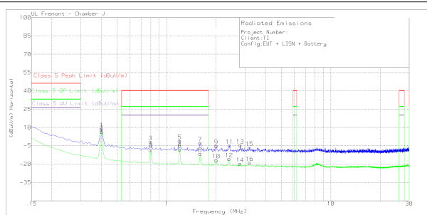
Figure 10-48. Radiated EMI Rod versus CISPR25 Limits
