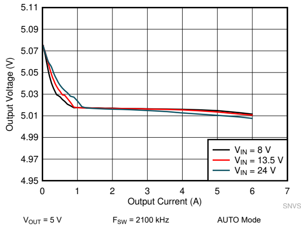
Figure 10-19. LM61460-Q1 Load and Line Regulation
