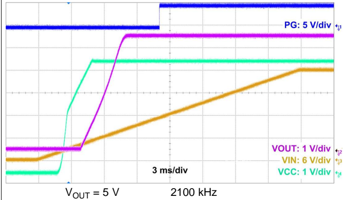
Figure 50. Start-Up Waveform
