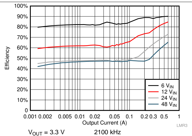
Figure 44. Efficiency
