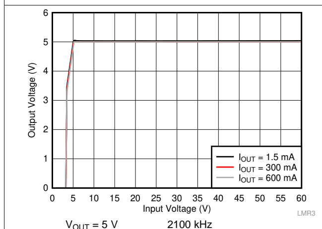
Figure 47. Line Regulation
