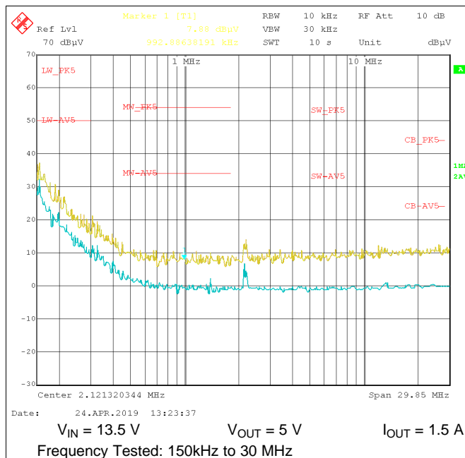
Figure 33. Conducted EMI vs. CISPR25 Limits (Yellow: Peak Signal, Blue: Average Signal)
