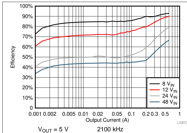
Figure 43. Efficiency
