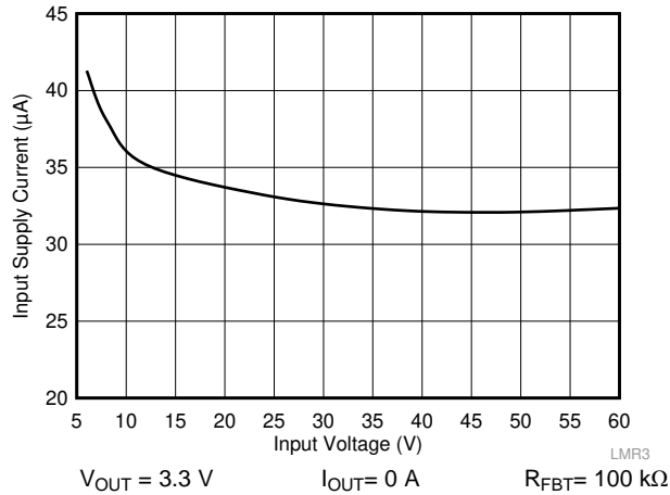
Figure 27. Input Supply Current
