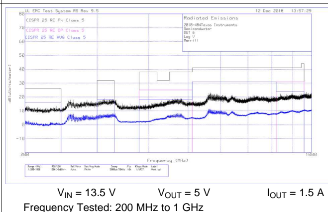
Figure 38. Radiated EMI Log Vertical vs. CISPR25 Limits
