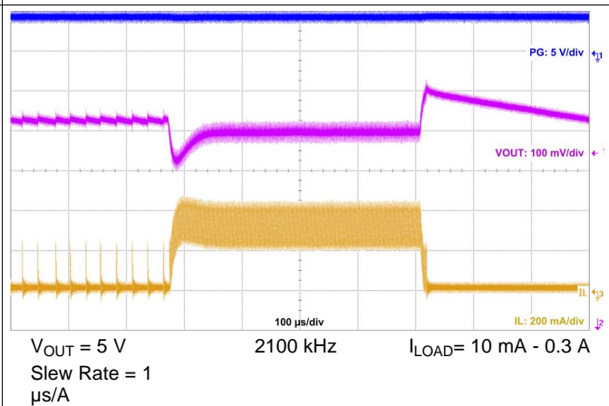
Figure 52. Load Transient
