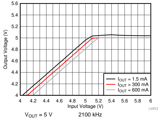
Figure 49. Overall Dropout Characteristic
