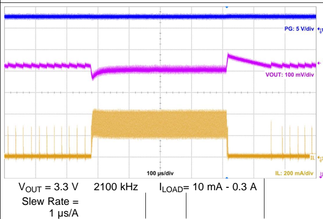
Figure 53. Load Transient
