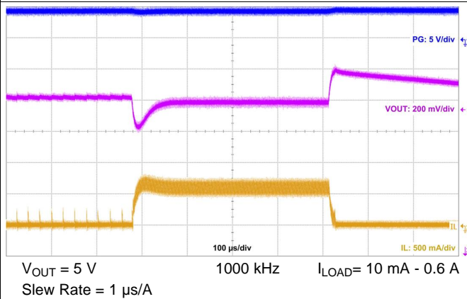
Figure 31. Load Transient
