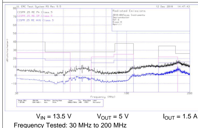
Figure 37. Radiated EMI Bicon Horizontal vs. CISPR25 Limits
