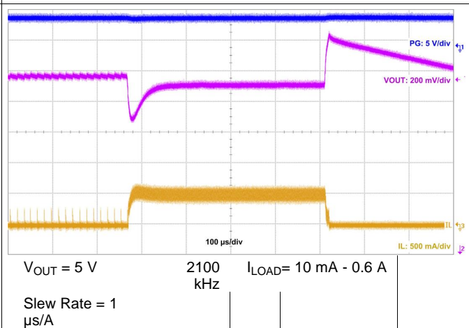
Figure 54. Load Transient
