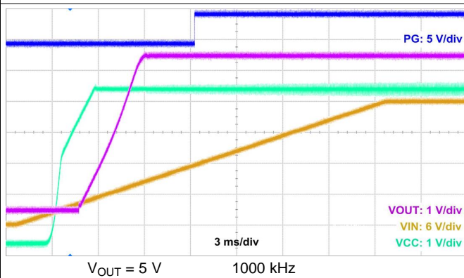
Figure 29. Start-Up Waveform
