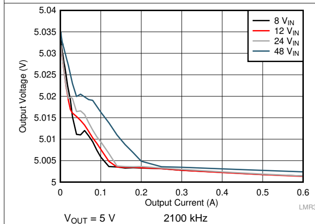
Figure 45. Load Regulation
