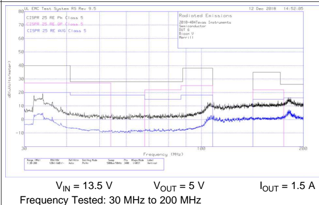
Figure 36. Radiated EMI Bicon Vertical vs. CISPR25 Limits
