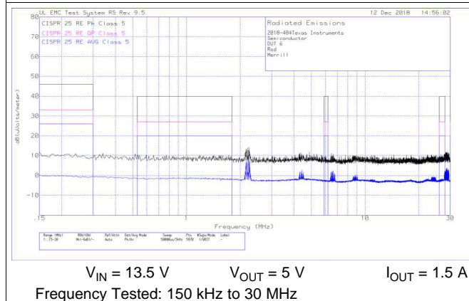
Figure 35. Radiated EMI Rod vs. CISPR25 Limits
