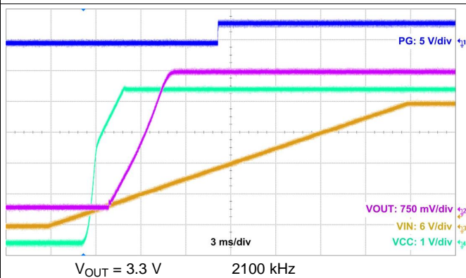
Figure 51. Start-Up Waveform
