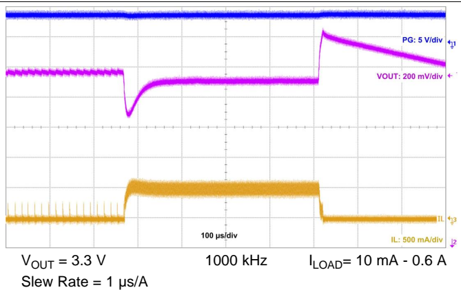
Figure 32. Load Transient
