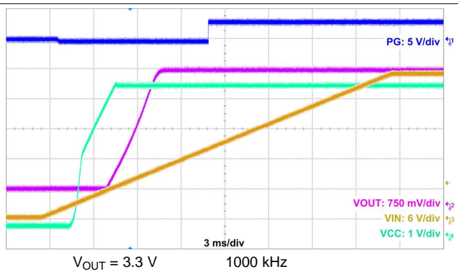
Figure 30. Start-Up Waveform
