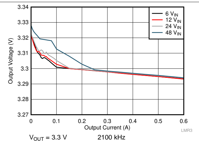
Figure 46. Load Regulation
