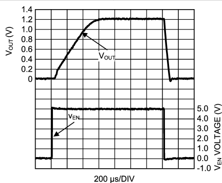
Figure 7-12. Enable - Disable
