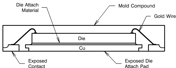
Figure 7-16. Internal Connection
