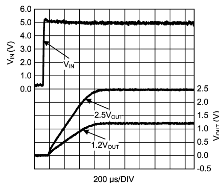
Figure 7-11. Start-Up (Soft Start)
