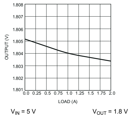
Figure 5-6. Load Regulation
