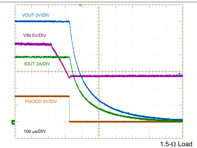
Figure 61. Shutdown Through Input UVLO, 8-A Resistive Load
