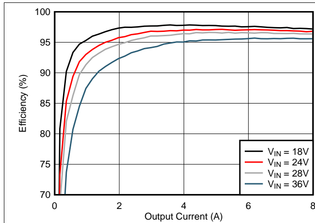
Figure 58. Efficiency vs I_{OUT} and V_{IN}
