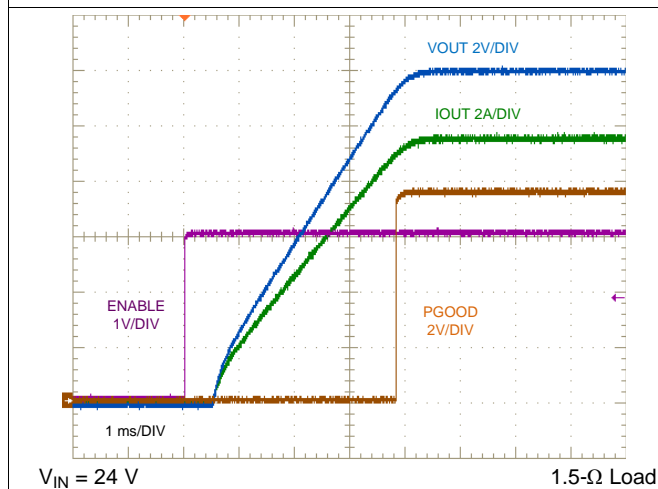
Figure 62. ENABLE ON, 8-A Resistive Load
