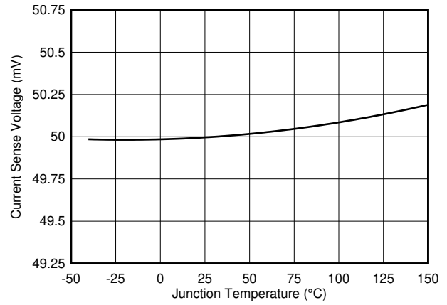
Figure 7-8. Regulated V_{CS} Voltage vs Temperature
