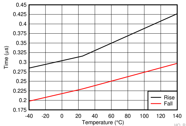
Figure 6-27. HO Rise &amp; Fall Time
