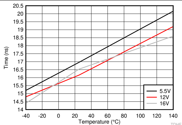
Figure 6-27. HO Rise &amp; Fall Time
