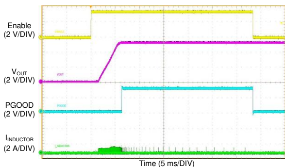
Figure 62. LM76003 Start-up Waveform
