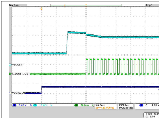
Figure 8-4. Typical Start-Up
