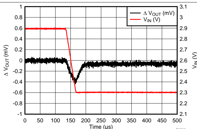
Figure 27. LP5912-0.9 Line Transient
