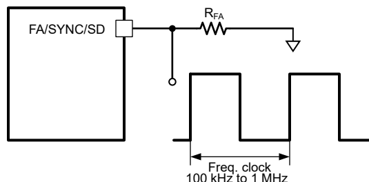
Figure 6-9. Frequency Synchronization
