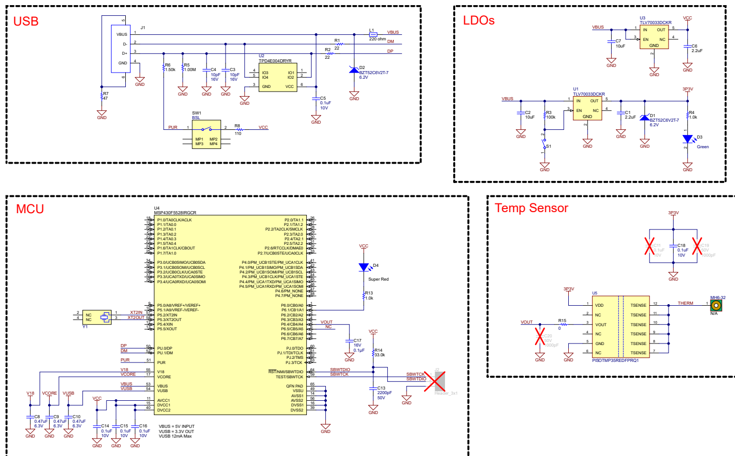
Figure 4-1. ISOTMP35REVM Schematic
