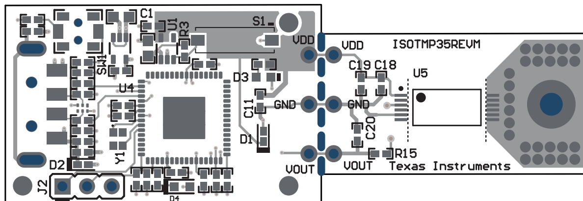
Figure 4-2. Top View
