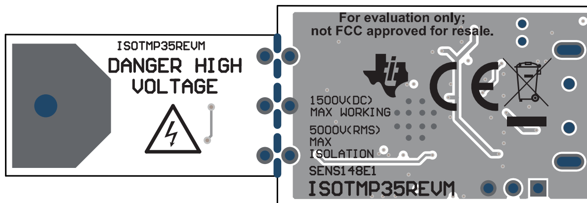
Figure 4-3. Bottom View
