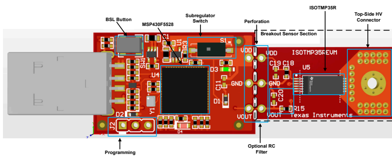
Figure 2-1. ISOTMP35REVM Board Top Side
