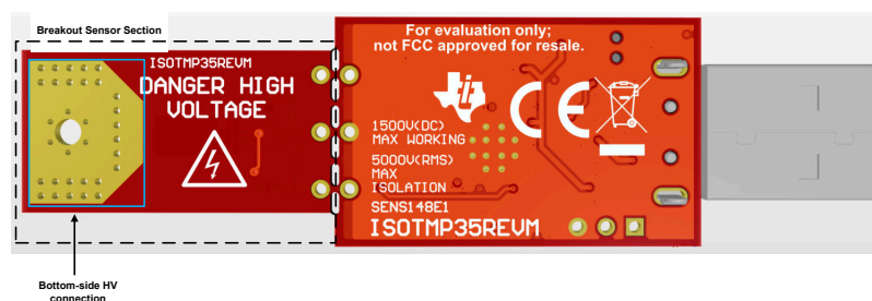
Figure 2-2. ISOTMP35REVM Board Bottom Side
