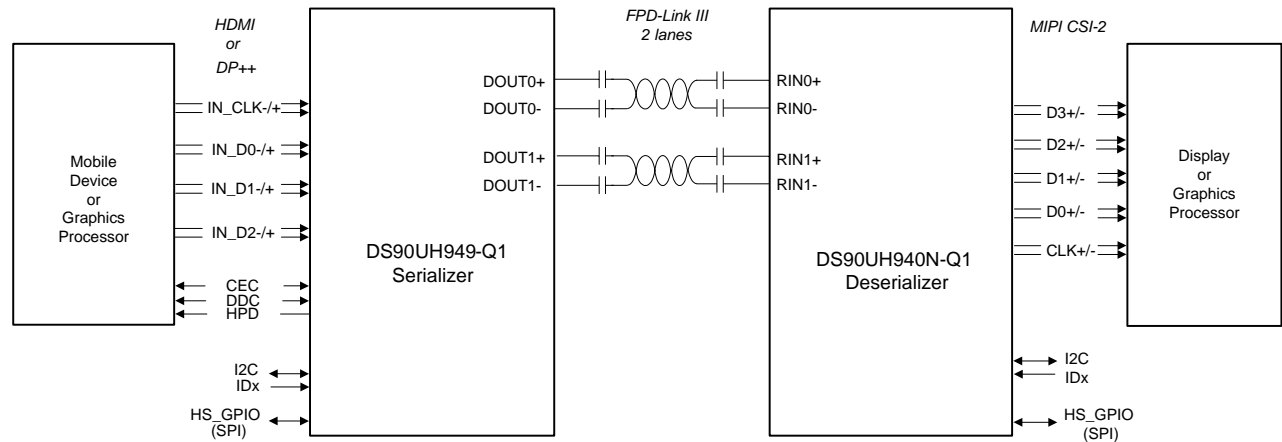
Figure 40. Typical Display System Diagram
