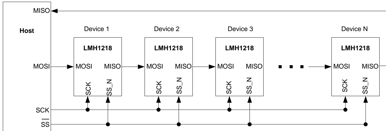
Figure 18. Daisy-Chain Configuration
