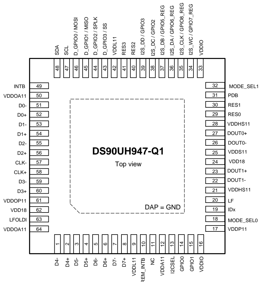
RGC Package 64-Pin VQFN Top View
