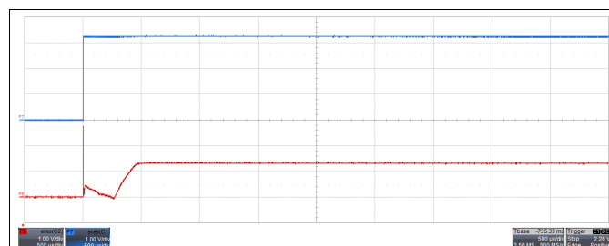
Figure 15. Output Turnon Response Time Without a Capacitive Load and V_{DD} = 3.3\text{ V}
