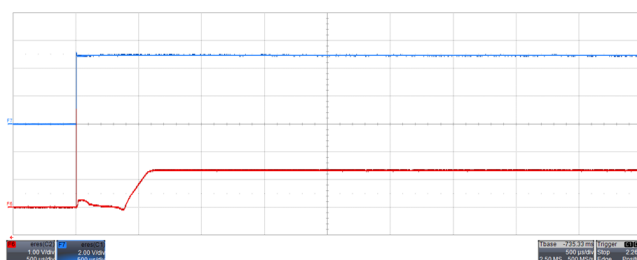
Figure 16. Output Turnon Response Time Without a Capacitive Load and V_{DD} = 5\text{ V}
