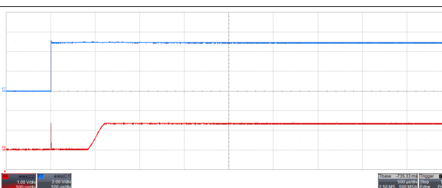
Figure 16. Output Turnon Response Time Without a Capacitive Load and V_{DD} = 5\text{ V}
