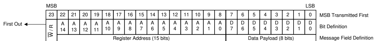
Figure 7-46. SPI Message Format
