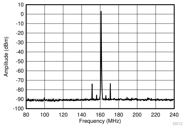
Figure 6-10. 161.1328125 ± 80.56640625-MHz LVPECL Differential Output Spectrum
