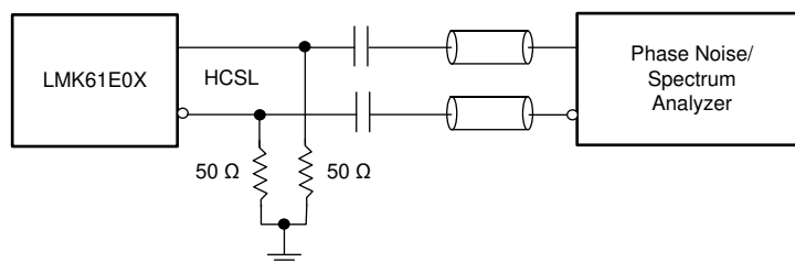
Figure 7-5. LVDS Output AC Configuration During Device Test
