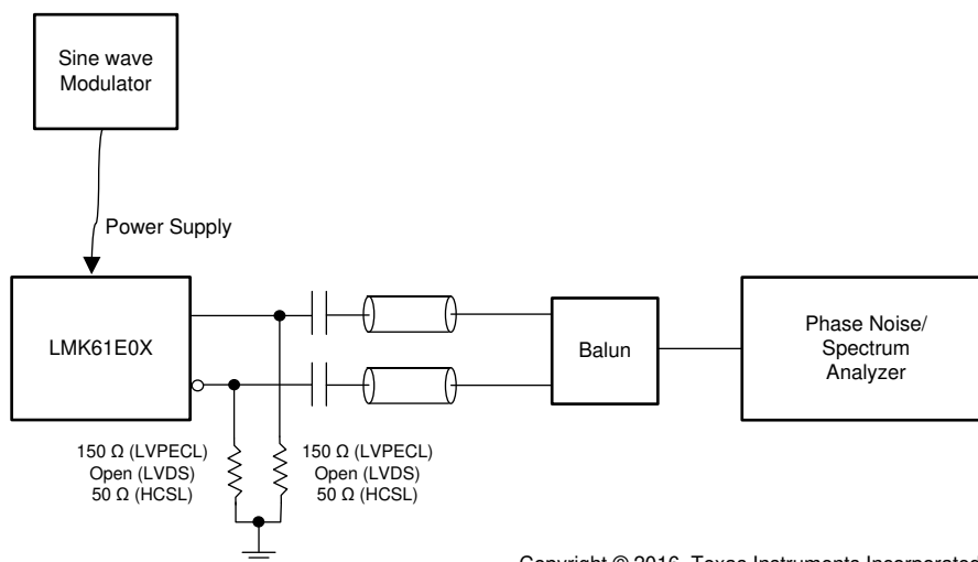
Figure 7-7. PSRR Test Setup
