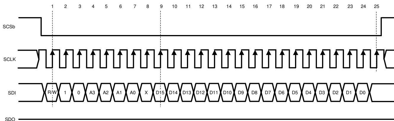
Figure 7-4. Serial Data Protocol - Write Operation
