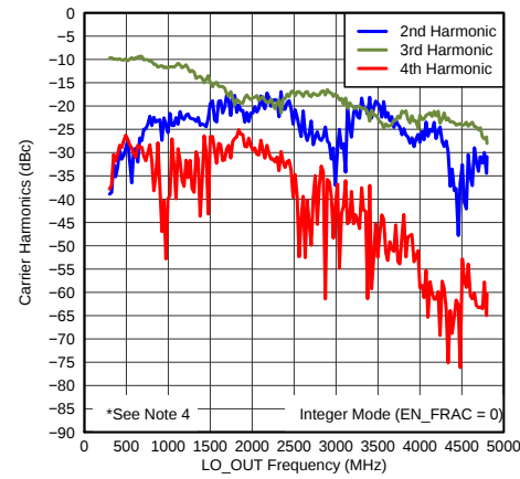
Figure 60. LO Harmonics
