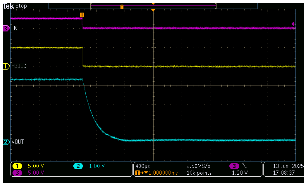
Figure 3-2. Shutdown Into 3.3Ω Load
