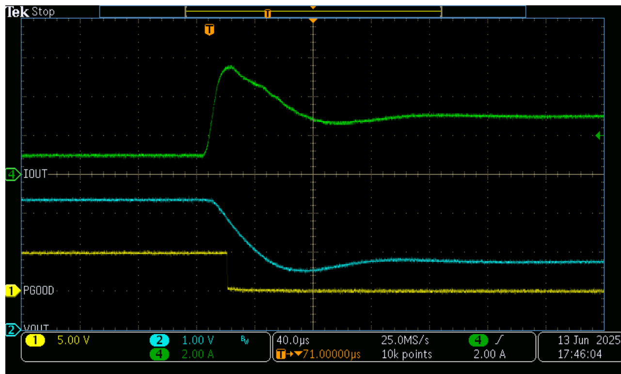
Figure 3-3. Current Limit Assertion - 3.3Ω to 0.55Ω Step
