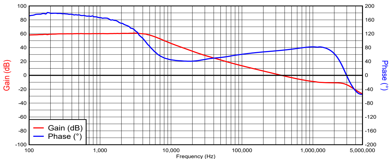
Figure 3-5. Frequency Response - IOUT = 2A
