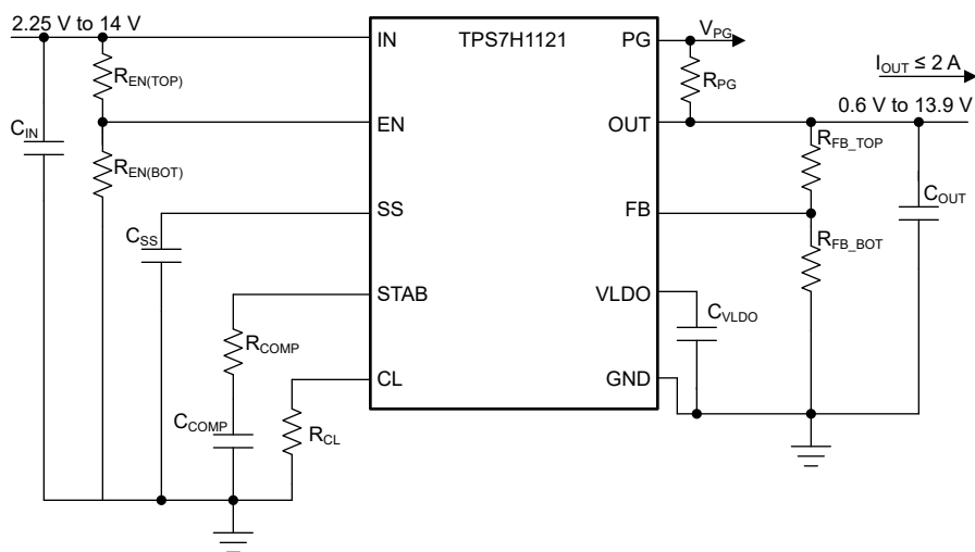
Figure 1-1. Simplified Schematic
