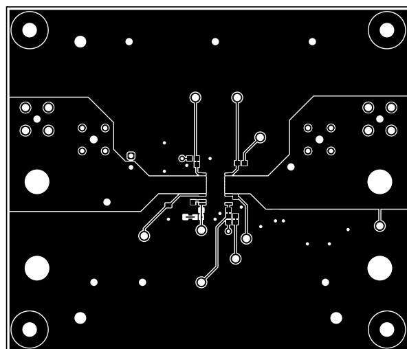
Figure 4-4. Layer 1 (Top)
