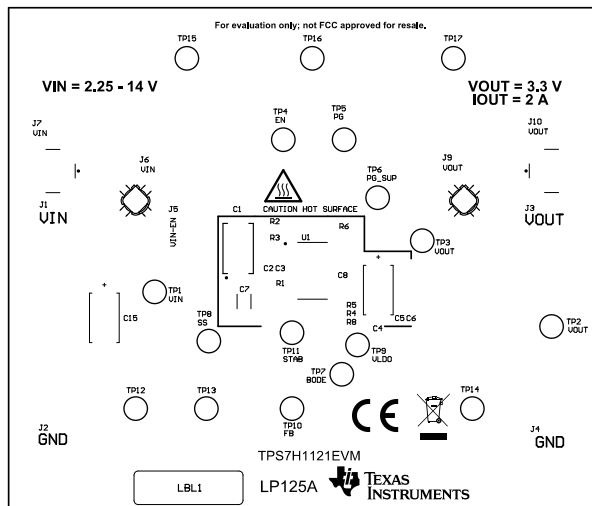
Figure 4-2. Top Overlay
