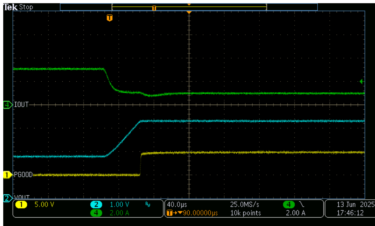
Figure 3-4. Current Limit Release - 0.55Ω to 3.3Ω Step
