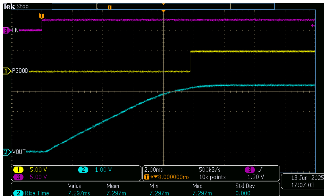
Figure 3-1. Soft Start Into 1.65Ω Load
