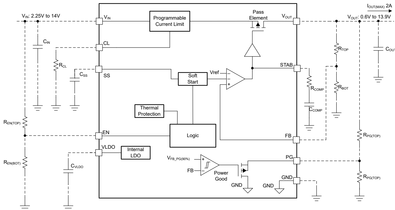
Figure 1-2. Functional Block Diagram
