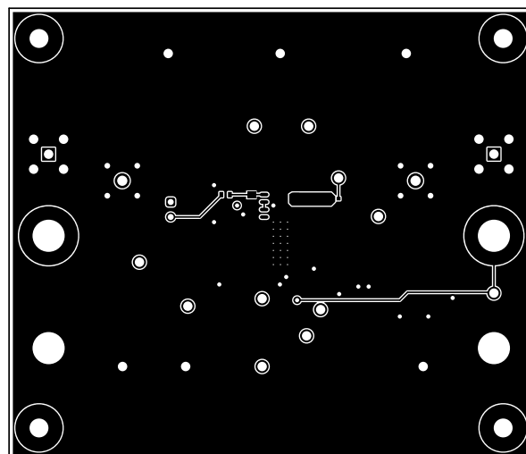
Figure 4-7. Layer 3 (Bottom)
