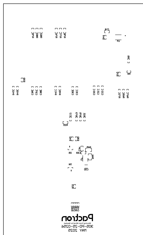
Figure 4-3. TPS1686-87EVM Board: Bottom Assembly
