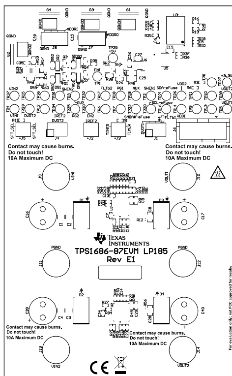
Figure 4-2. TPS1686-87EVM Board: Top Assembly
