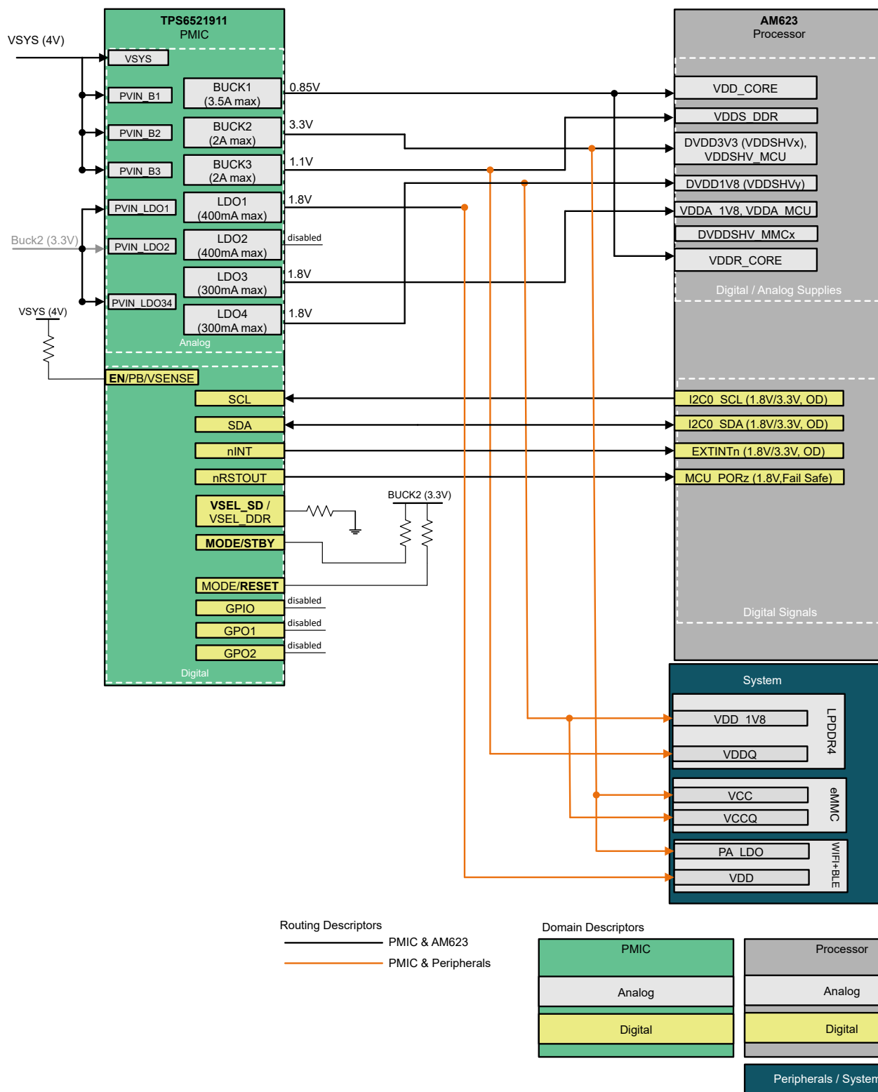
Figure 2-1. TPS6521911 Example Power Block Diagram
