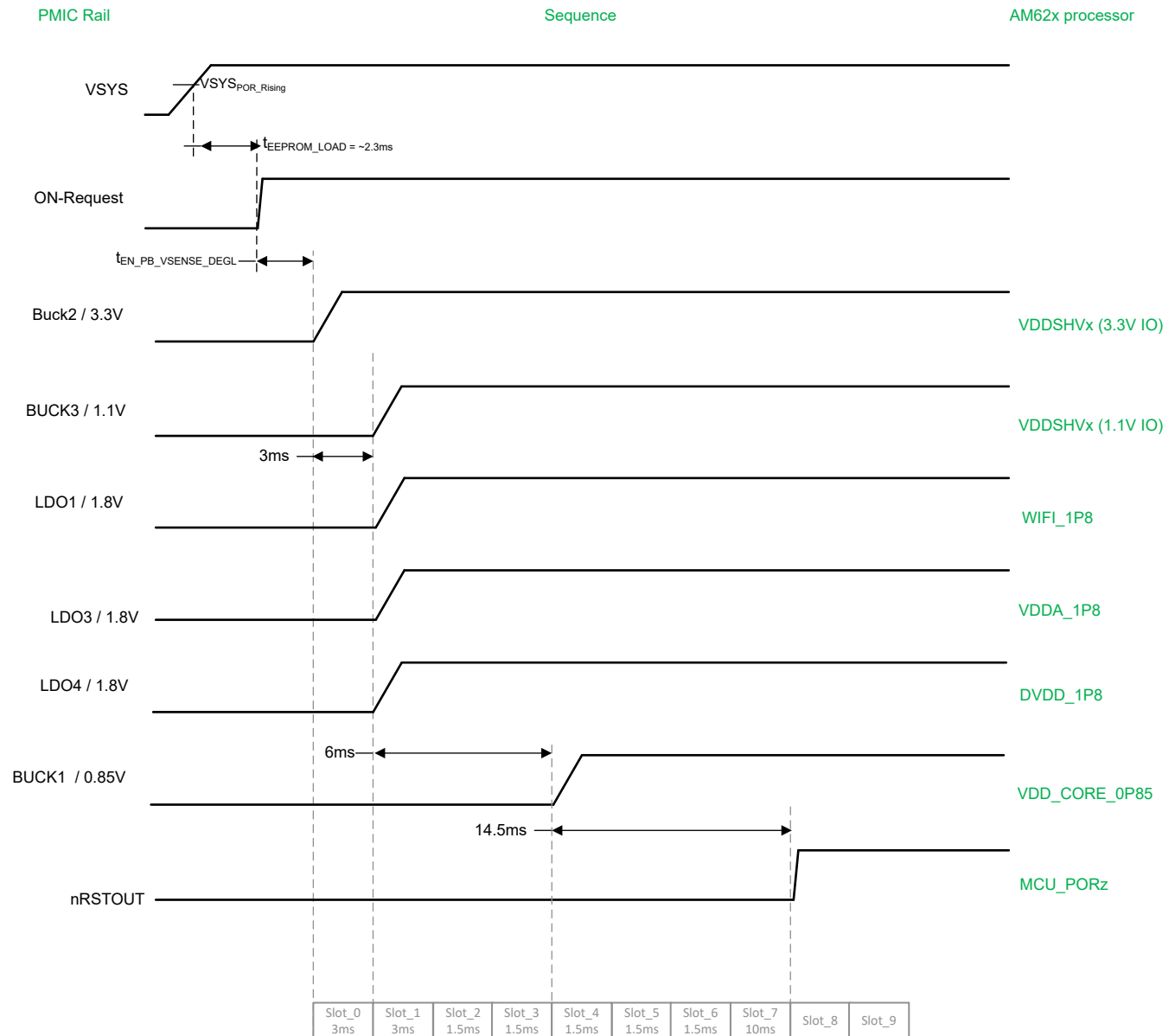
Figure 2-2. TPS6521911 Power-Up Sequence
