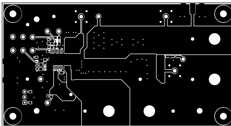
Figure 4-4. Layer 1 (Top)
