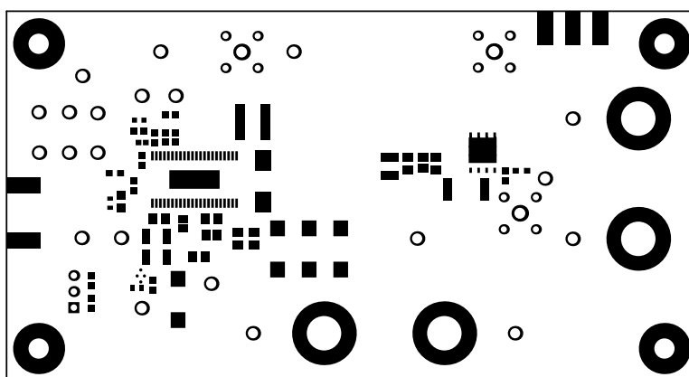
Figure 4-3. Top Solder Mask
