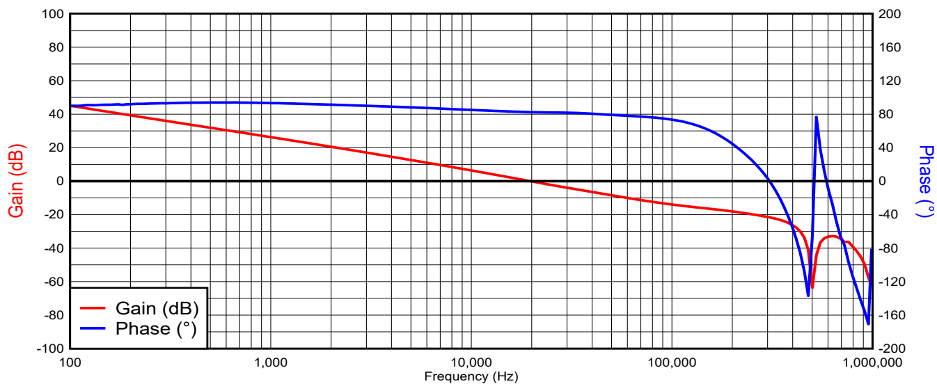
Figure 3-5. Frequency Response IOUT = 3A
