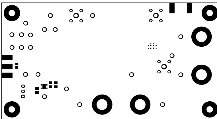
Figure 4-8. Bottom Solder Mask
