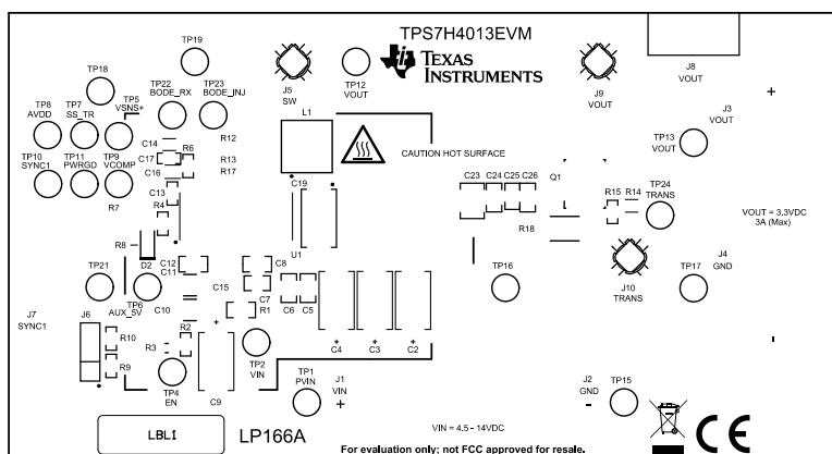
Figure 4-2. Top Overlay
