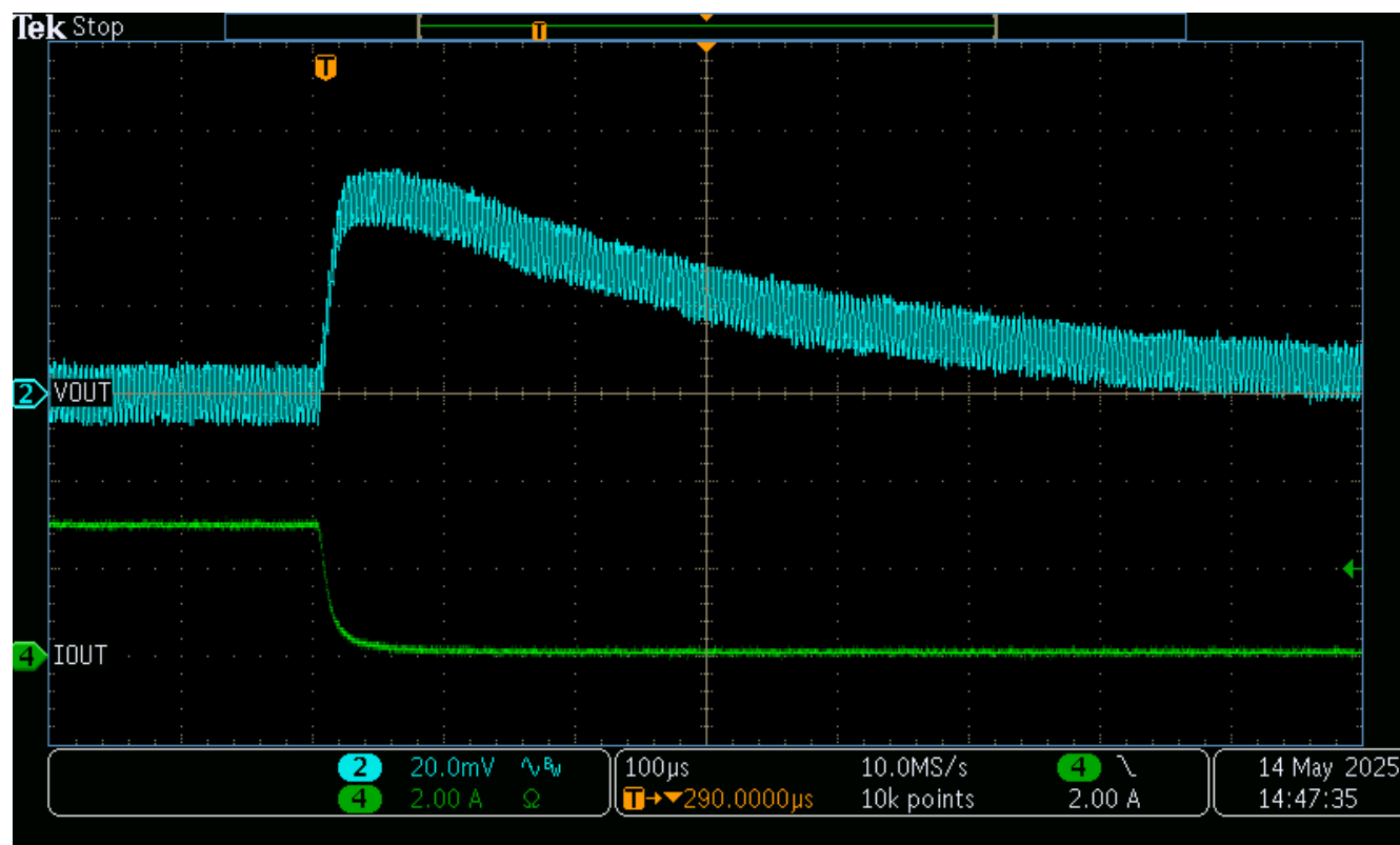
Figure 3-4. Transiant Response to Load Step 3A to 100mA at 8A/μs
