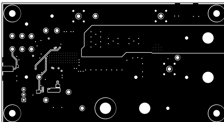
Figure 4-7. Layer 4 (Bottom)
