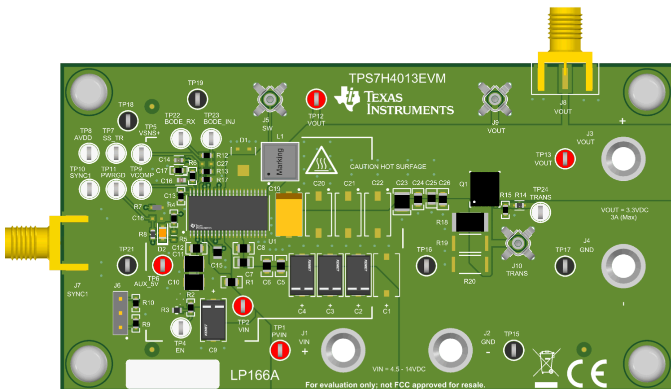
EVM Board
