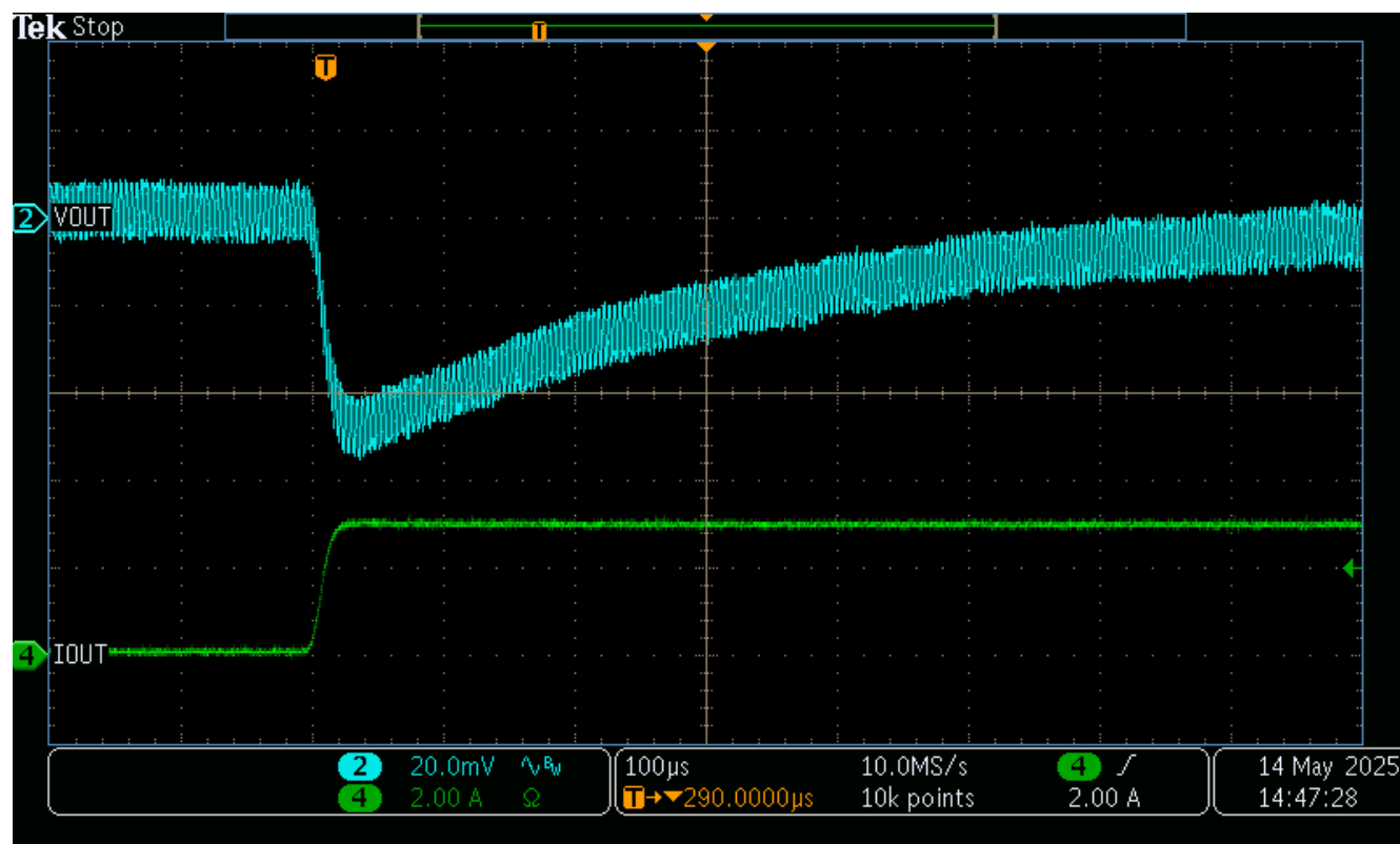
Figure 3-3. Transiant Response to Load Step 100mA to 3A at 8A/μs
