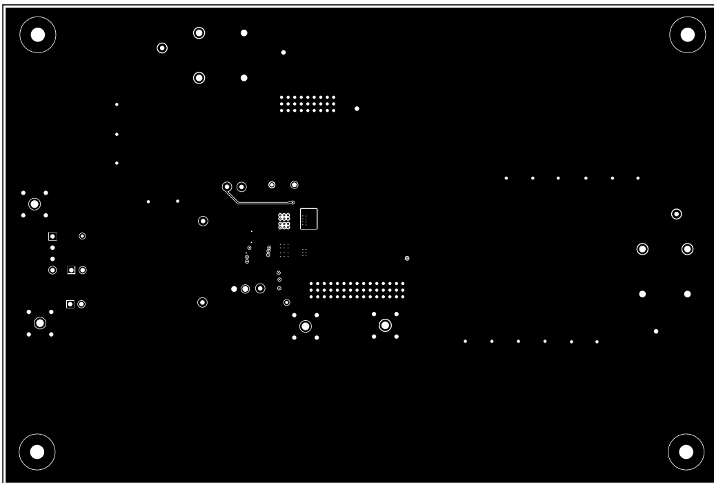
Figure 4-8. Signal Layer 3 (TPS7H6101EVM)
