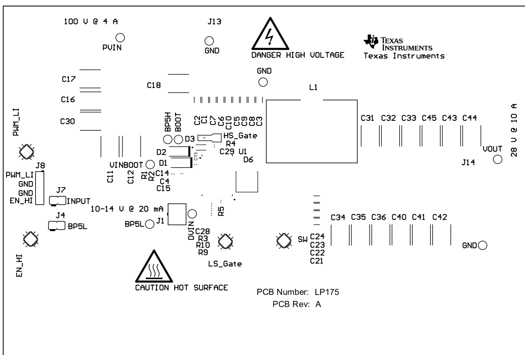
Figure 4-4. Top Overlay (TPS7H6101EVM)
