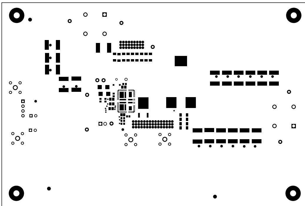
Figure 4-3. Top Solder Mask (TPS7H6101EVM)
