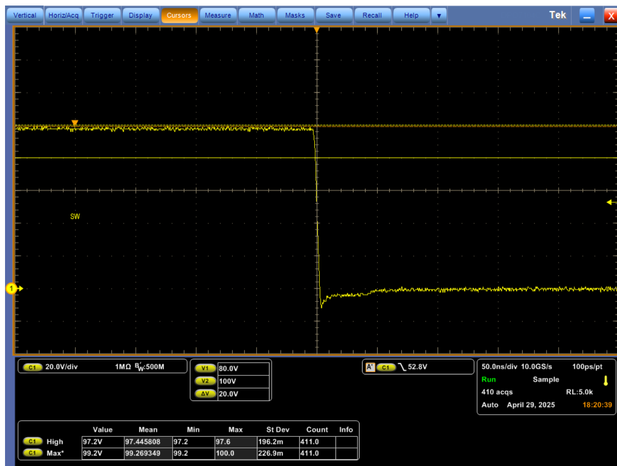
Figure 3-5. Switch Node Falling Transition
