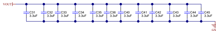
Figure 4-2. TPS7H6101EVM Schematic, Page 2
