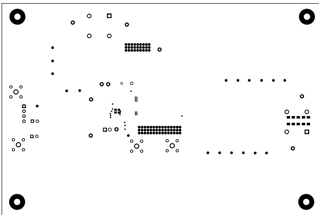
Figure 4-14. Bottom Solder (TPS7H6101EVM)
