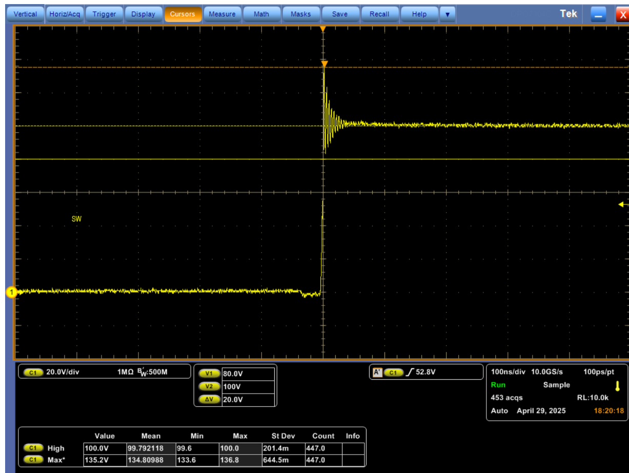
Figure 3-4. Switch Node Rising Transition
