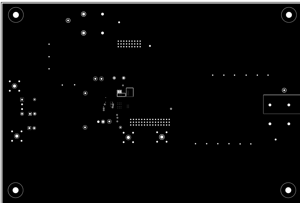
Figure 4-12. Bottom Layer (TPS7H6101EVM)
