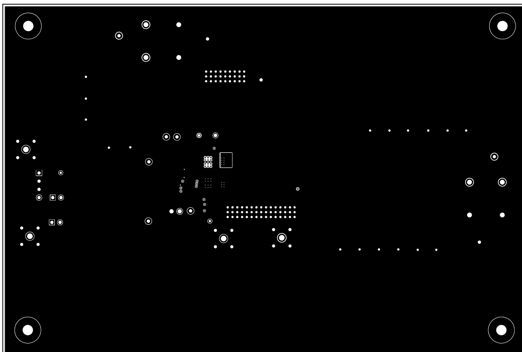
Figure 4-9. Signal Layer 4 (TPS7H6101EVM)
