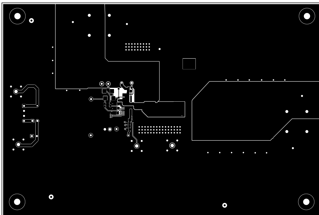
Figure 4-5. Top Layer (TPS7H6101EVM)
