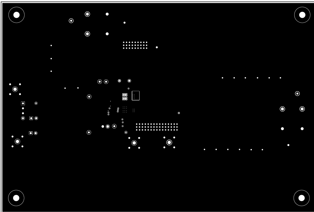
Figure 4-11. Signal Layer 6 (TPS7H6101EVM)
