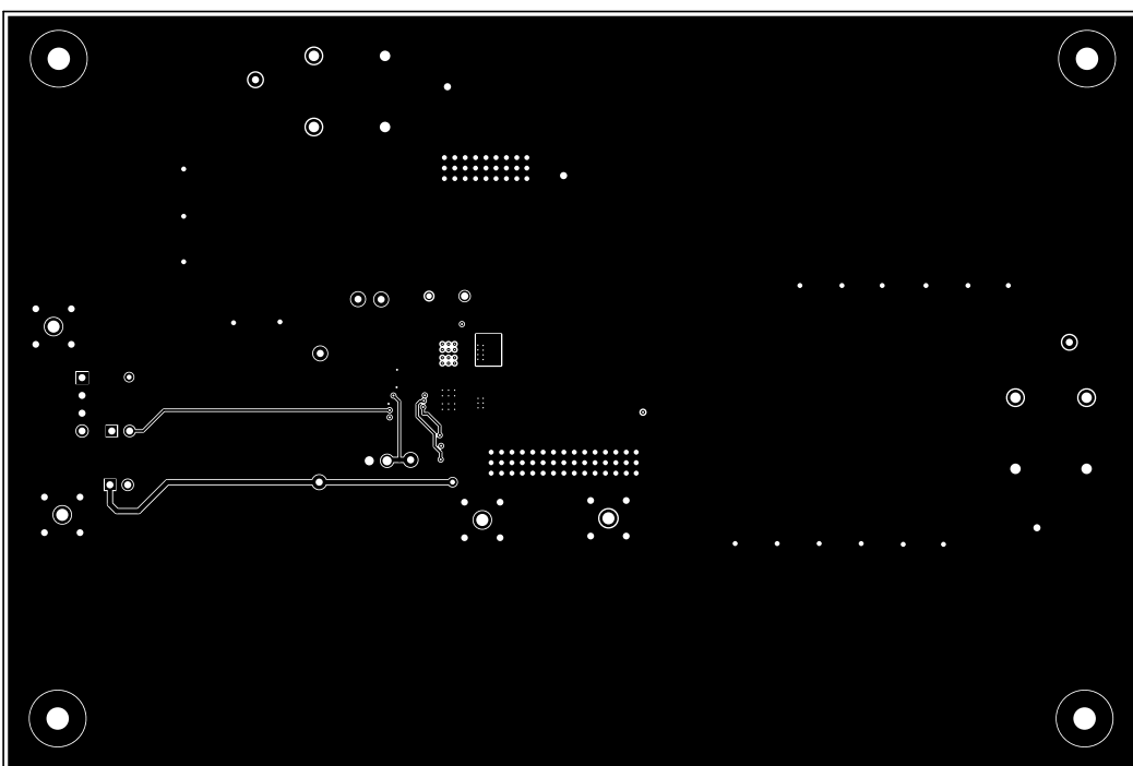
Figure 4-6. Signal Layer 1 (TPS7H6101EVM)
