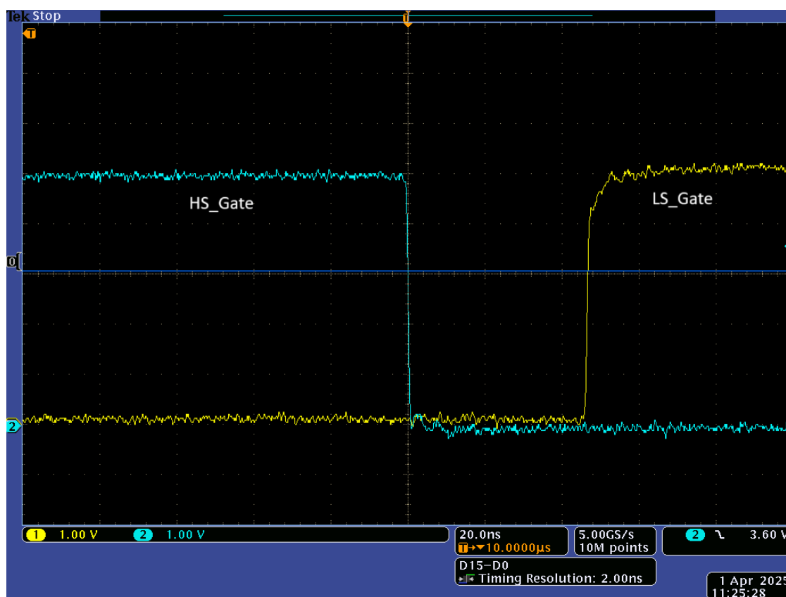
Figure 3-1. High to Low Transition of Gate Voltage
