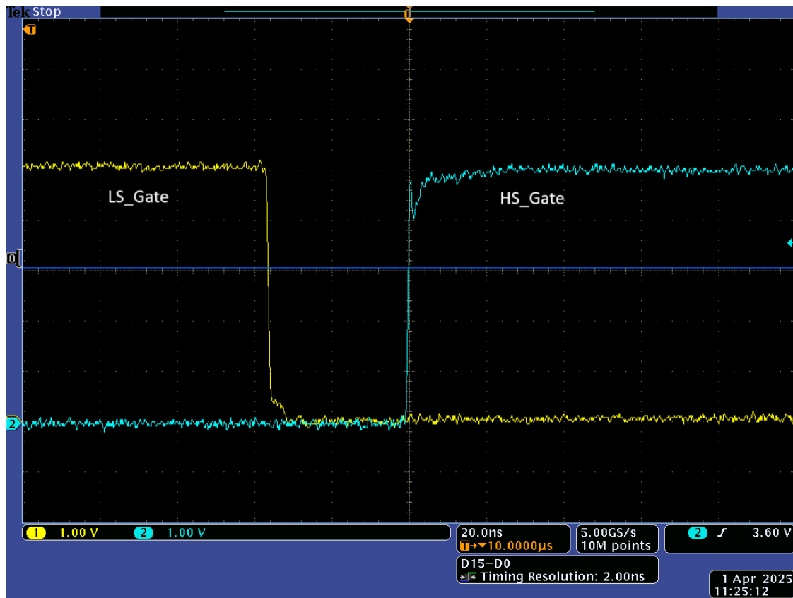
Figure 3-2. Low to High Transition of Gate Voltage
