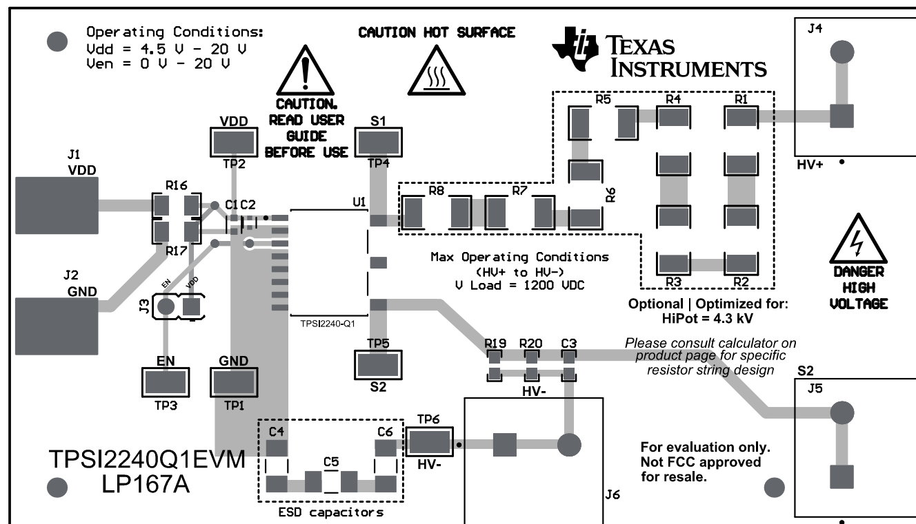
Figure 4-2. TPSI2240-Q1 EVM - Composite View
