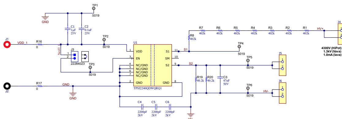
Figure 4-1. TPSI2240Q1EVM Schematic
