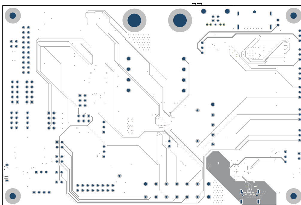
Figure 5-11. GND1 Layer (2)
