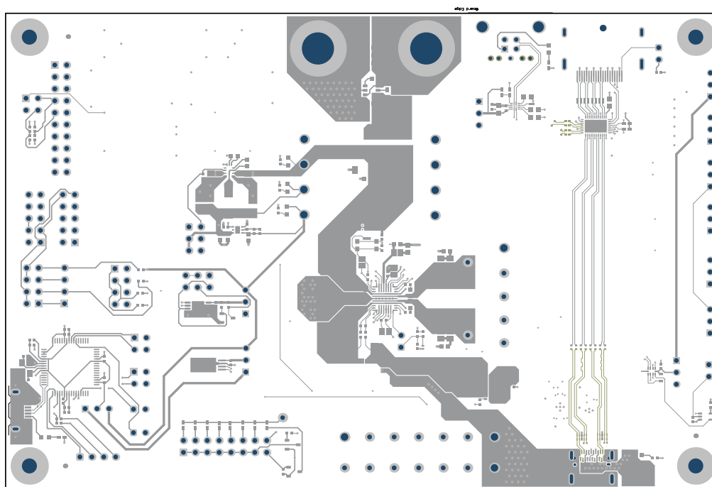
Figure 5-9. Bottom Composite View
