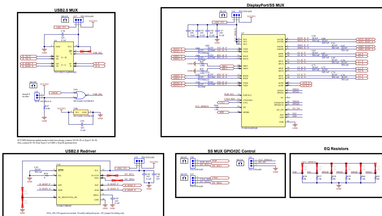
Figure 5-4. Data, Display Port MUX
