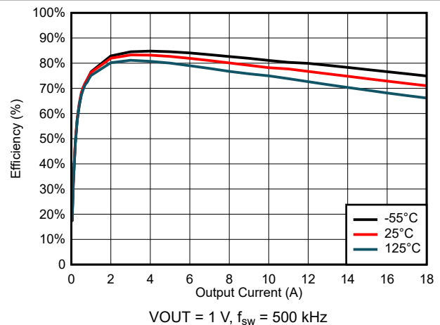
Figure 6-30. Efficiency for VIN = 7 V
