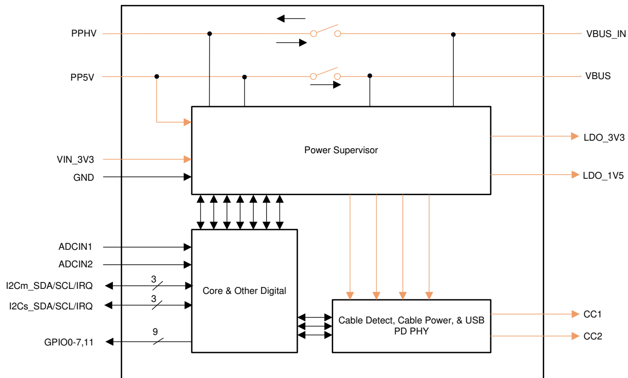
Figure 9-1. TPS25750D
