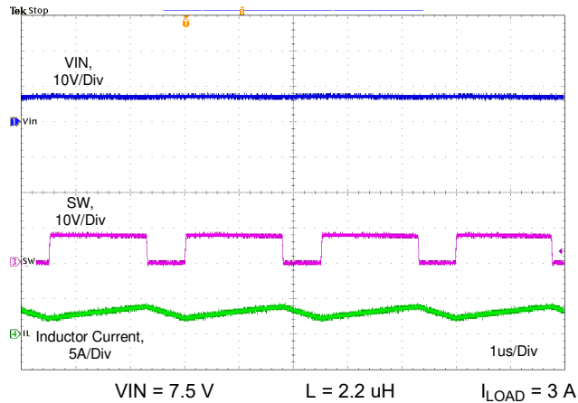
Figure 10-7. Switching Frequency when R_T = 8.87 k \Omega
