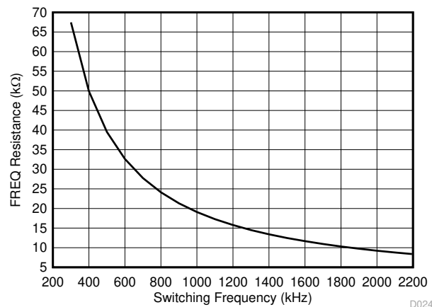
Figure 10-5. RT Set Resistor vs Switching Frequency
