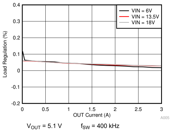
Figure 11-6. Load Regulation
