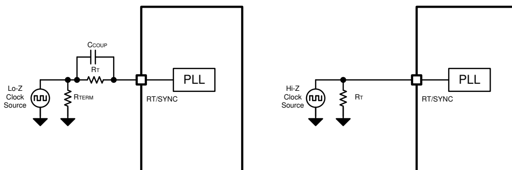
Figure 10-6. Synchronize to External Clock
