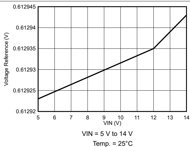
Figure 7-14. Voltage Reference Variation
