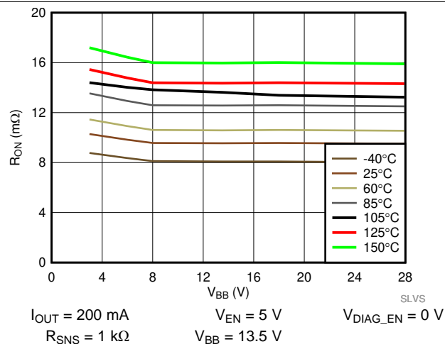
Figure 8. On Resistance ( R_{ON} ) vs V_{BB}
