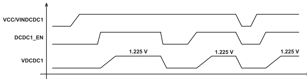
Figure 38. Default DCDC1
