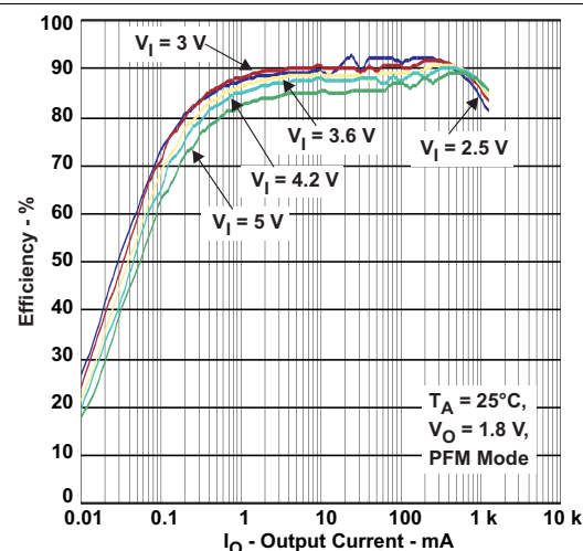
Figure 45. DCDC2: Efficiency vs Output Current
