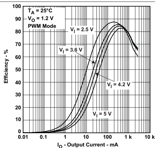
Figure 3. DCDC1: Efficiency vs Output Current
