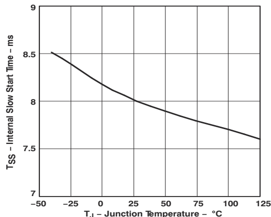
Figure 6-6. Internal Slow Start Time vs Junction Temperature
