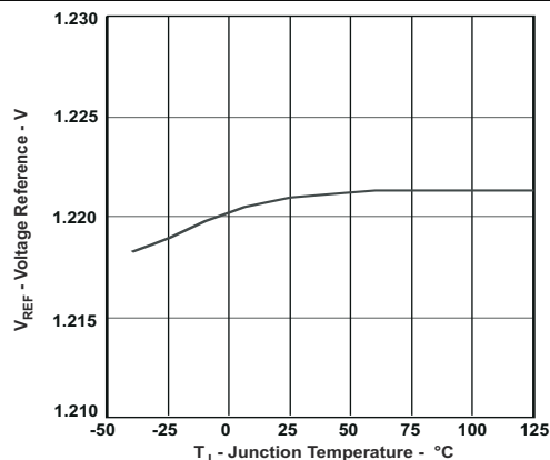
Figure 6-4. Voltage Reference vs Junction Temperature
