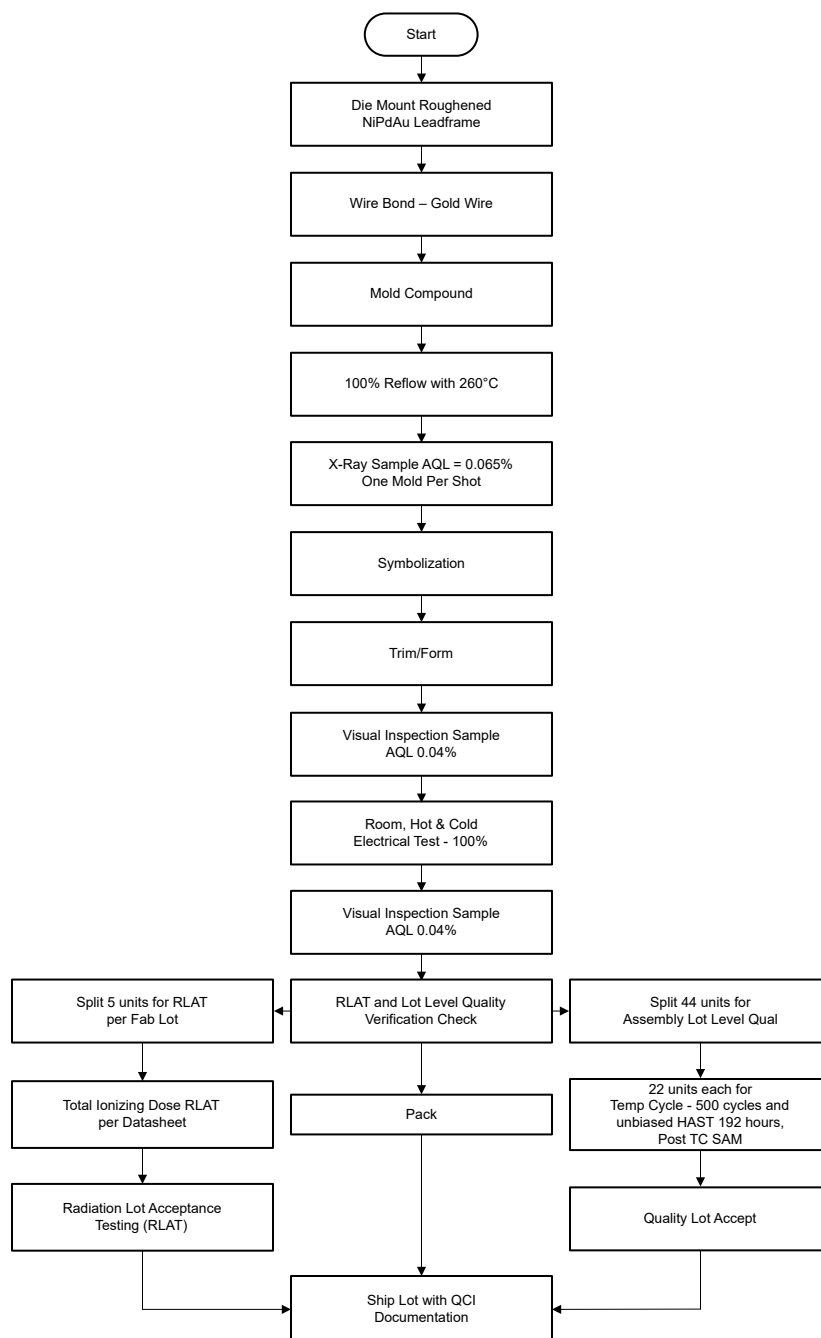
Figure 1-1. ISOS141-SEP Space Enhanced Plastic Production Flow Chart
