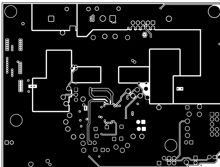
Figure 4-8. Signal Layer 2
