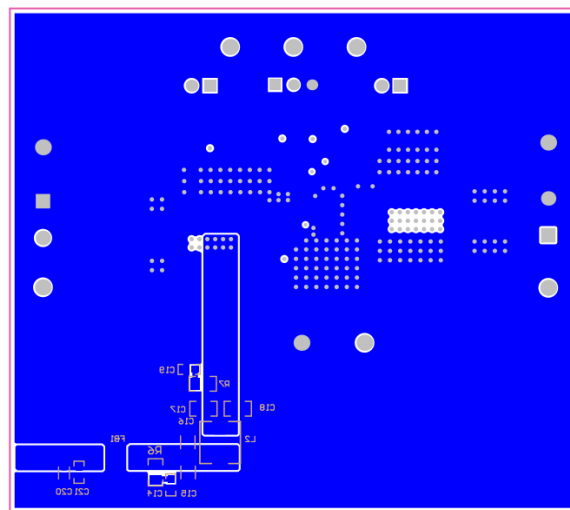
Figure 3-5. Bottom Copper (Top View)
