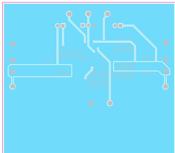
Figure 3-4. Layer 3 Copper (Top View)
