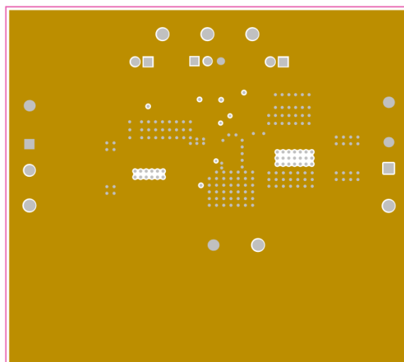
Figure 3-3. Layer 2 Copper (Top View)
