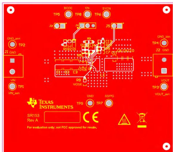
Figure 3-2. Top Copper (Top View)
