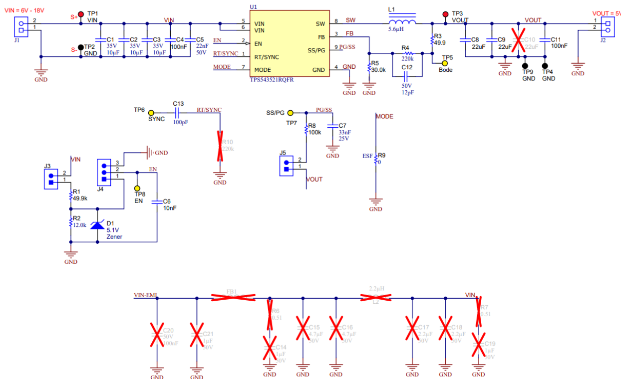
Figure 3-1. TPS543521EVM Schematic Diagram
