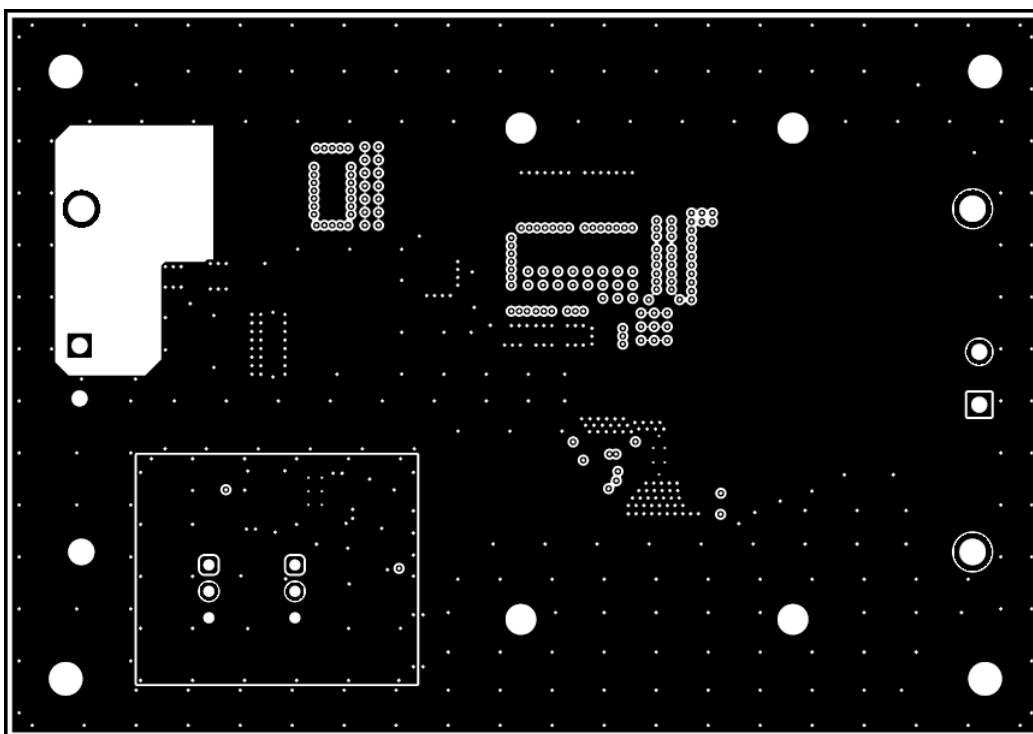
Figure 7-4. TPS922055DMTREV Bottom Layer
