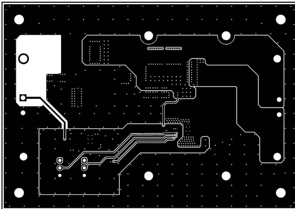
Figure 7-3. TPS922055DMTREV Inner Layer 2
