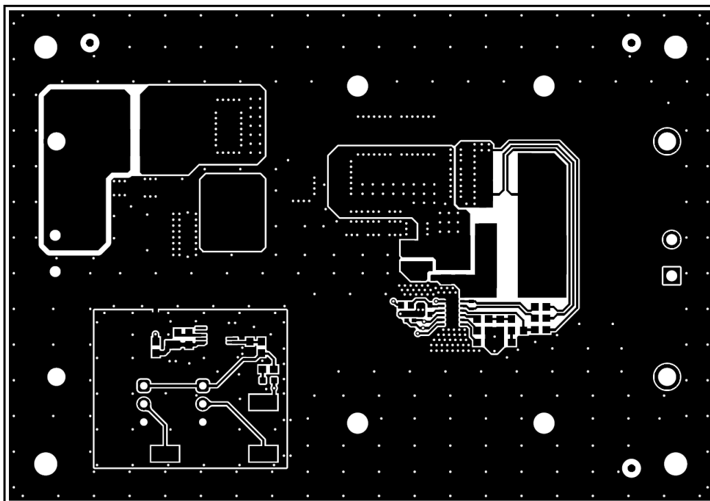
Figure 7-1. TPS922055DMTREVMM Top Layer
