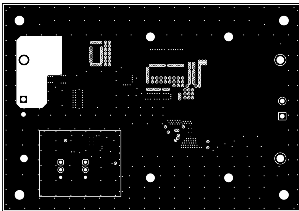
Figure 7-2. TPS922055DMTREVMM Inner Layer 1
