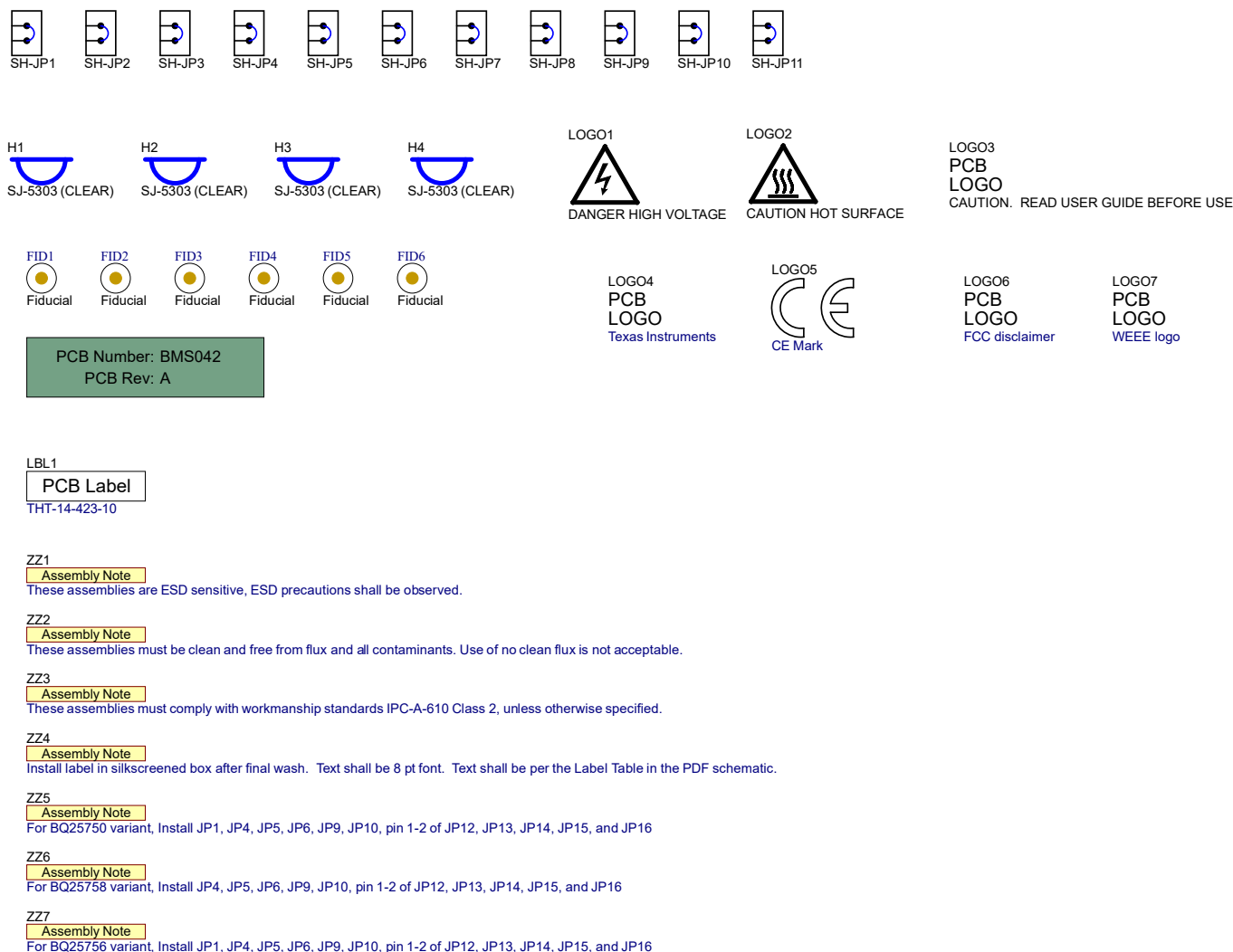
Figure 3-4. BQ25758 and BQ25758A EVM Schematic Page
