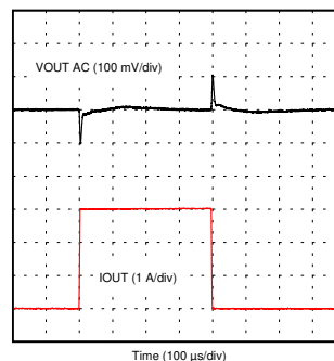
Figure 8-32. Load Transient
